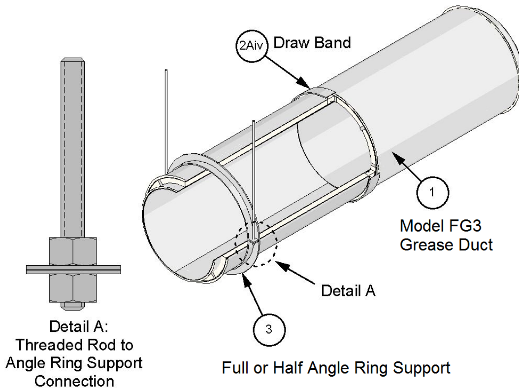
Figure 1. Model FG3
