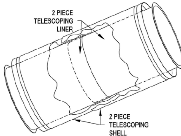
Figure 4. Adjustable Length (AL) Section and Joint
