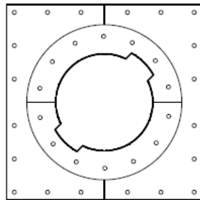
Figure 7. Support Plate, Part No. SP
