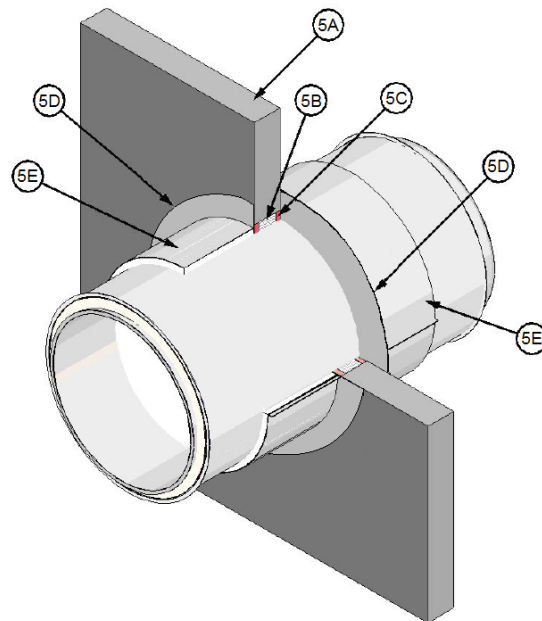
Figure 9. Wall Firestop
