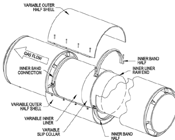
Figure 3. Variable Straight (VS) Length Section and Joint
