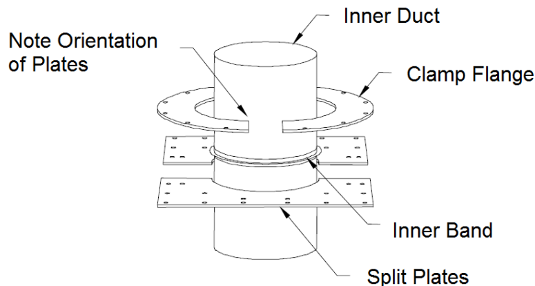
Figure 5. Support Plate, Part No. SP – Exploded View
