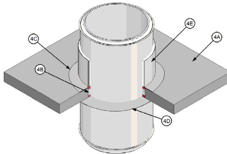
Figure 8: Floor/Ceiling Firestop
