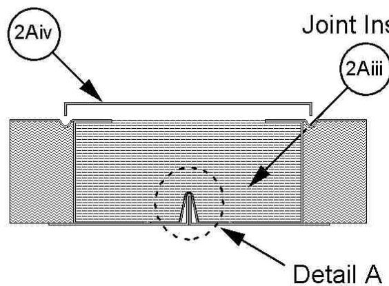
Figure 2. Standard Joint
