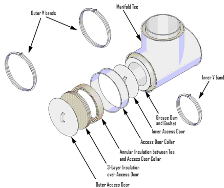
Figure 2. Access Door Assembly
