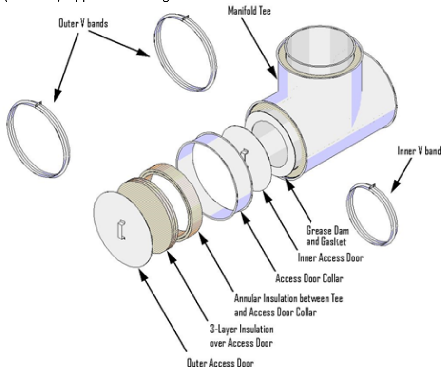
Figure 2. Access Door Assembly
