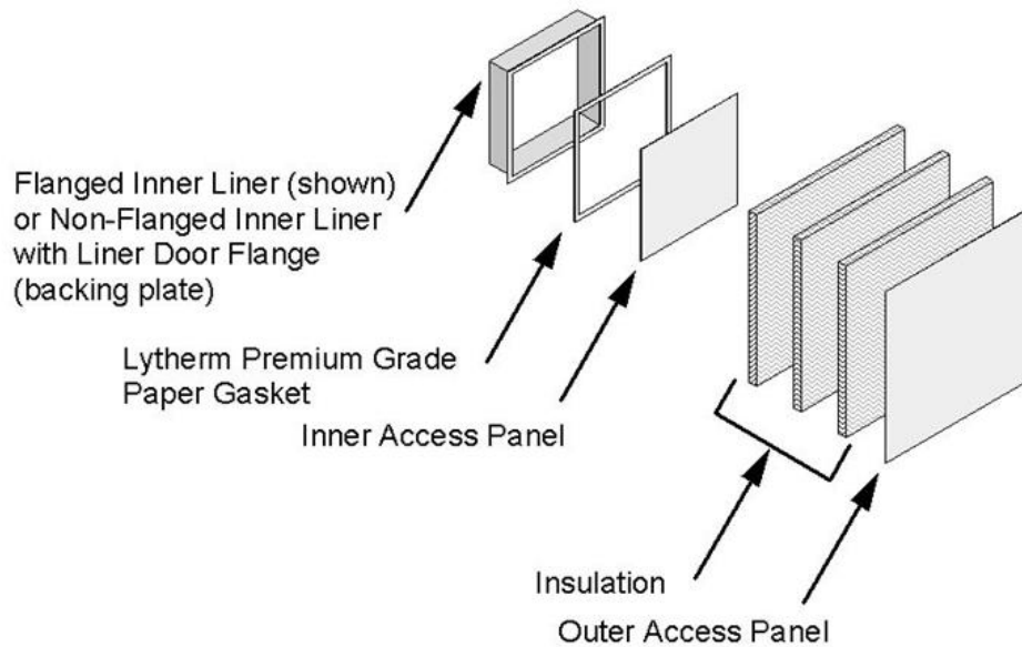
Figure 2. Access Door
