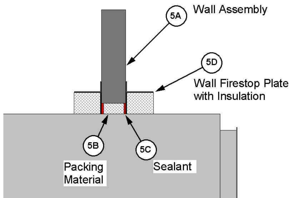
Figure 7. Wall Firestop
