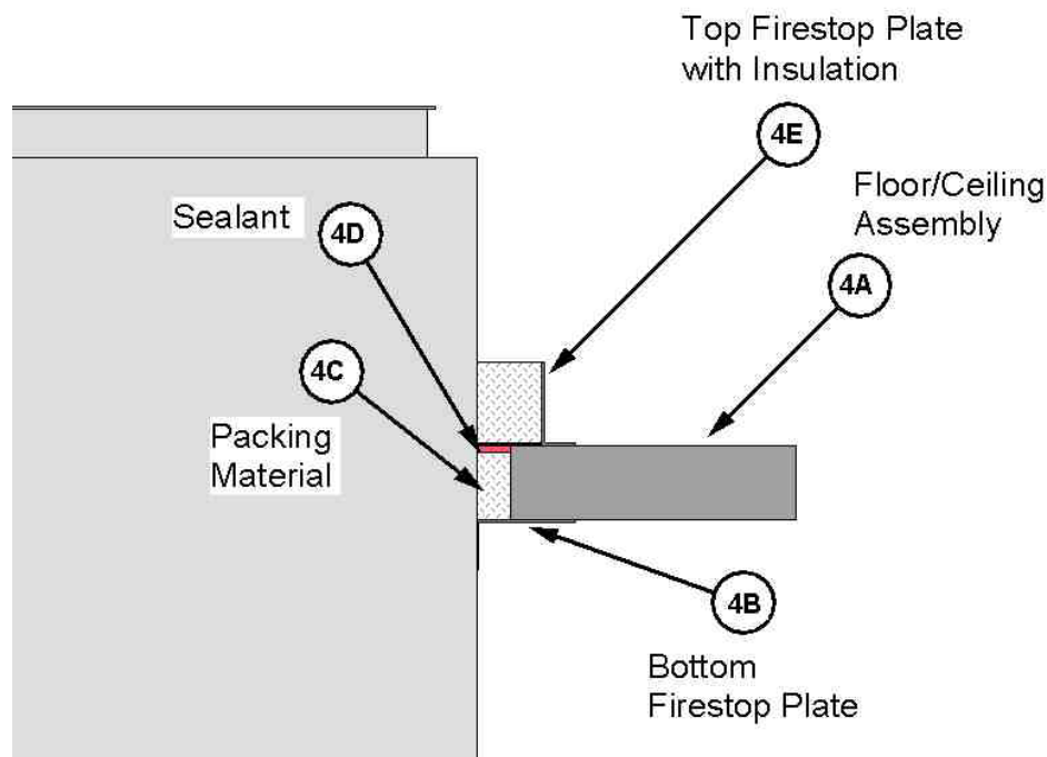
Figure 6. Floor/Ceiling Firestop
