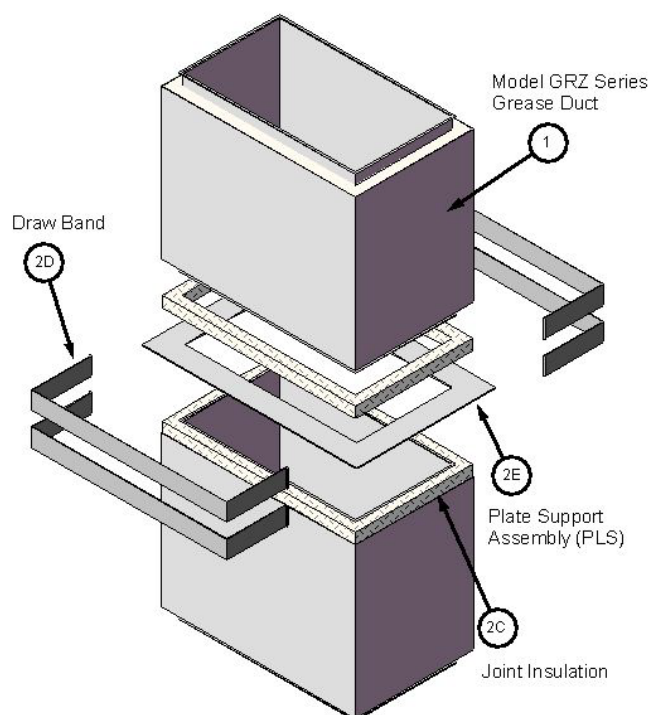
Figure 3. Plate Support Assembly (PLS)
