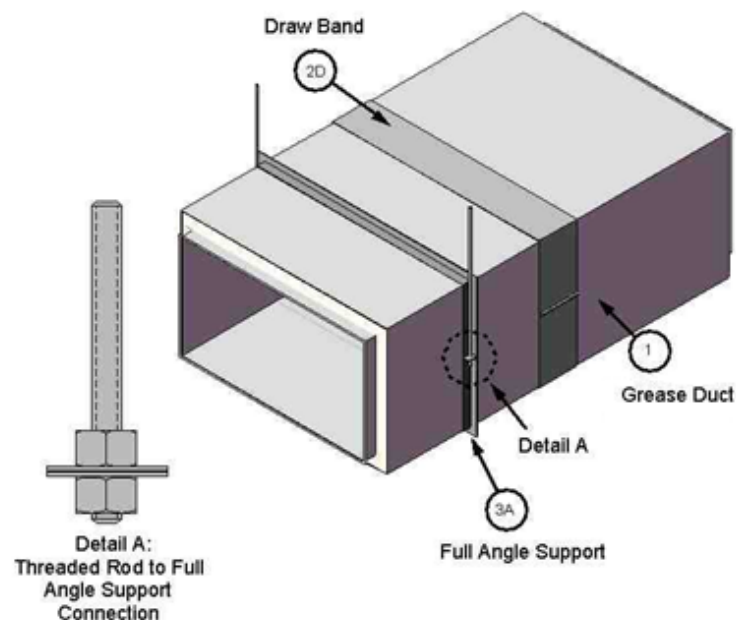
Figure 1. Model DWGD-RZ Grease Duct
