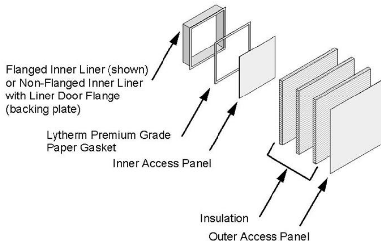
Figure 2. Access Door
