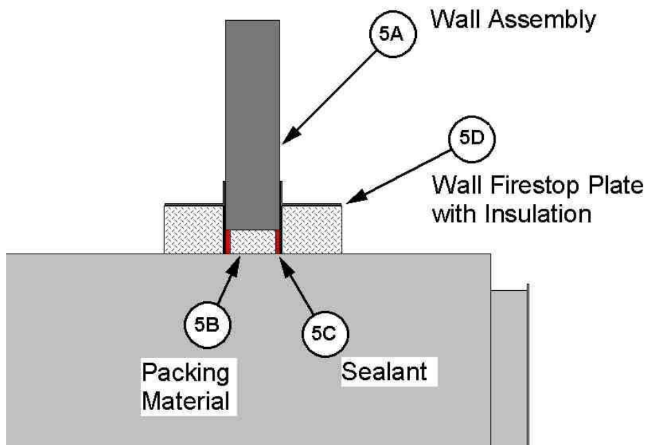
Figure 7. Wall Firestop
