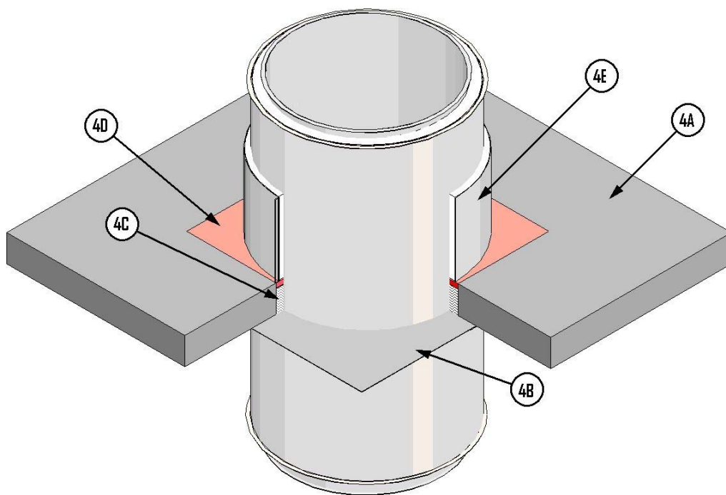
Figure 4: Floor/Ceiling Firestop
