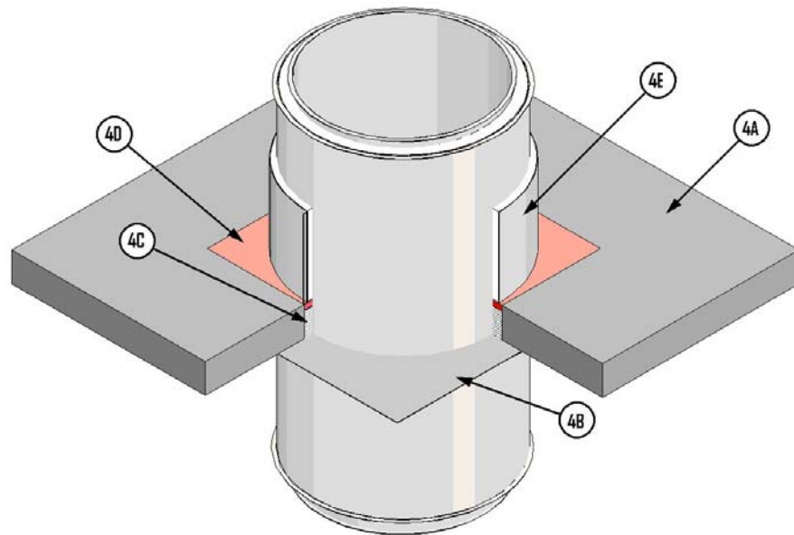
Figure 6: Floor/Ceiling Firestop
