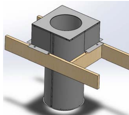
Curb Vertical Support
