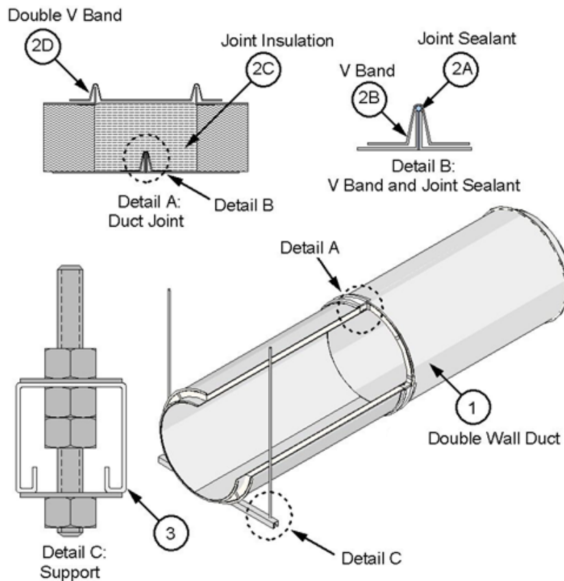
Figure 1. Double Wall Duct and Horizontal Support
