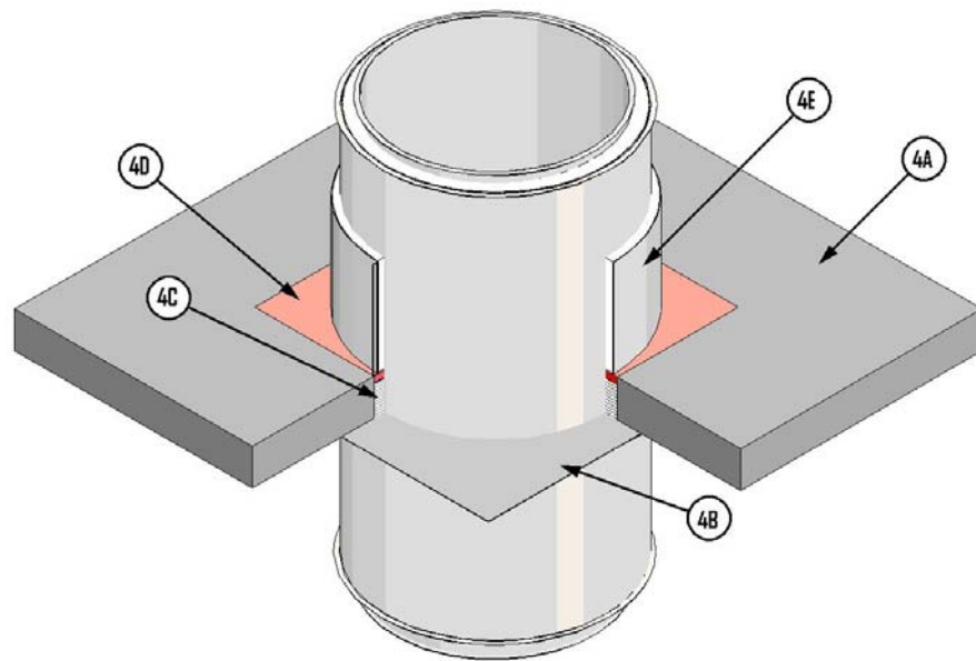
Figure 6: Floor/Ceiling Firestop
