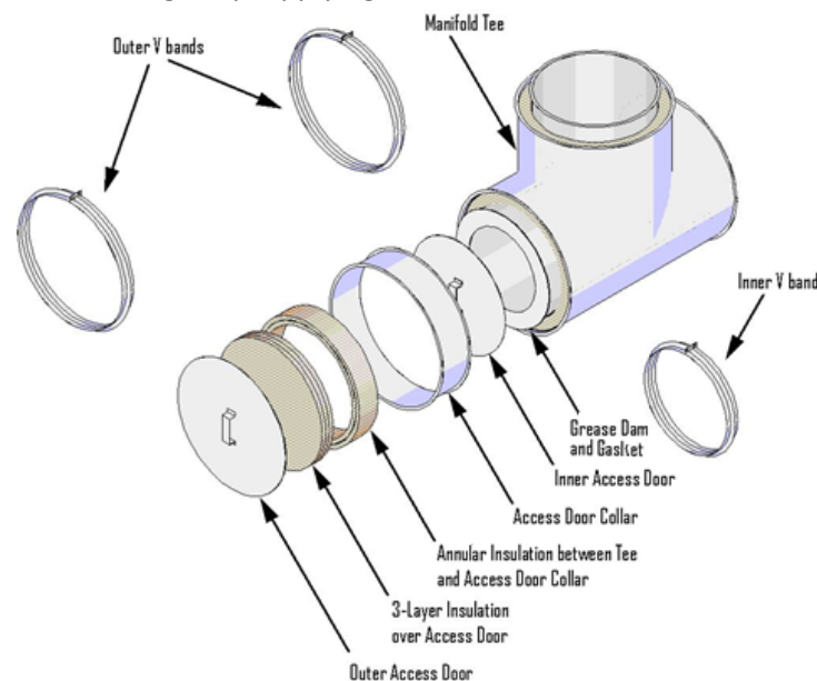
Figure 2. Access Door Assembly
