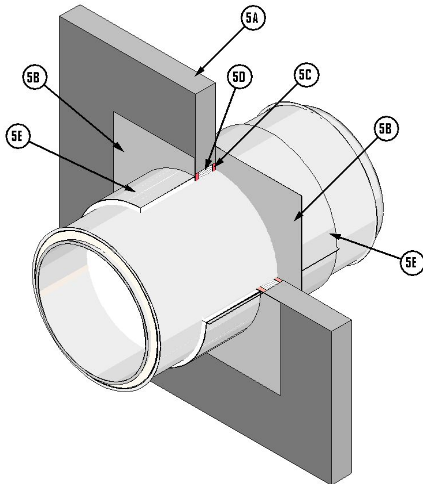
Figure 5. Wall Firestop
