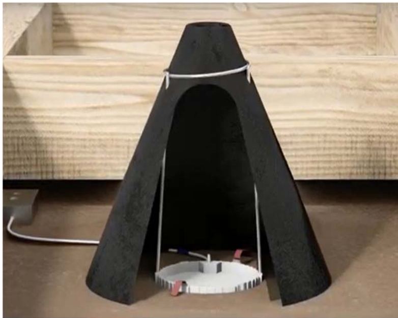
Figure 2. FF109-200 with Bronze Wire – Installation Example with LED fixture
