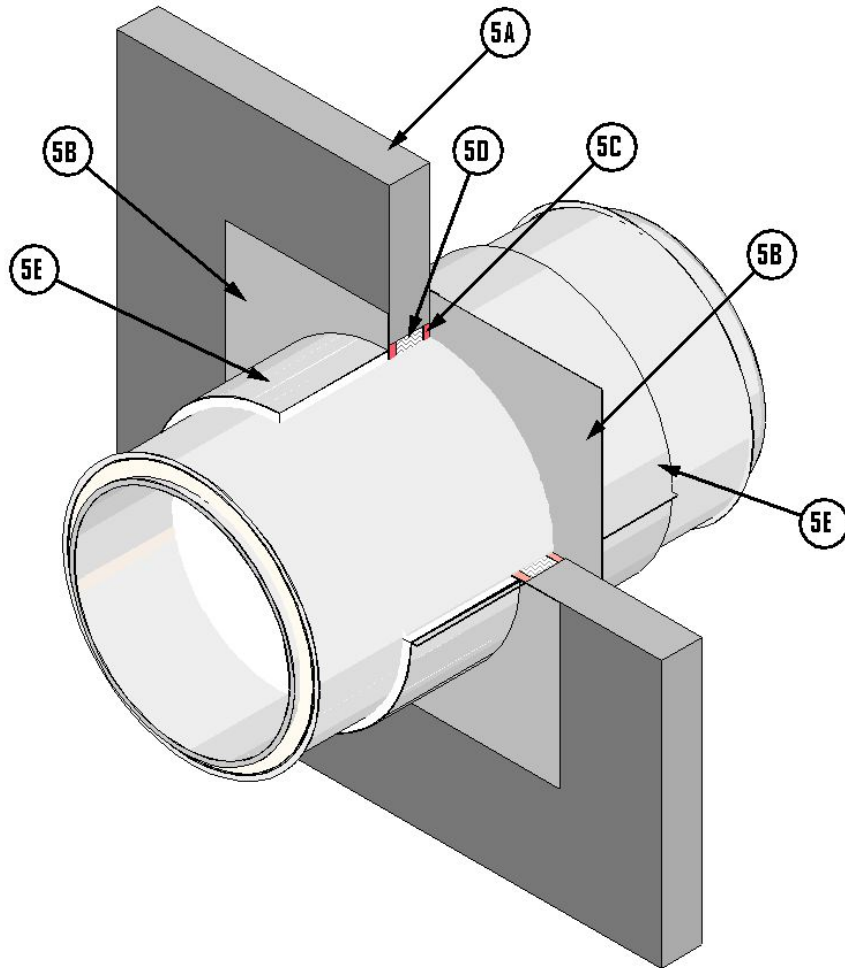
Figure 5. Wall Firestop
