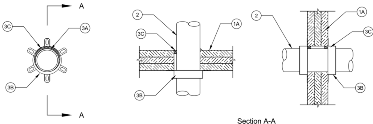
Figure 1. Through Penetration Detail
