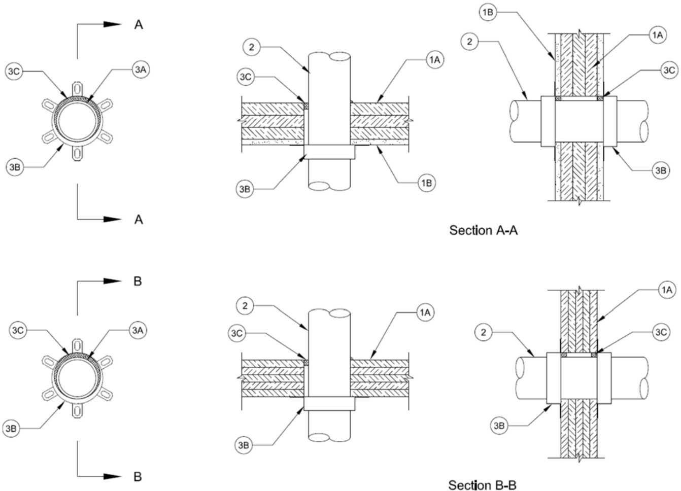
Figure 1. Through Penetration Detail
