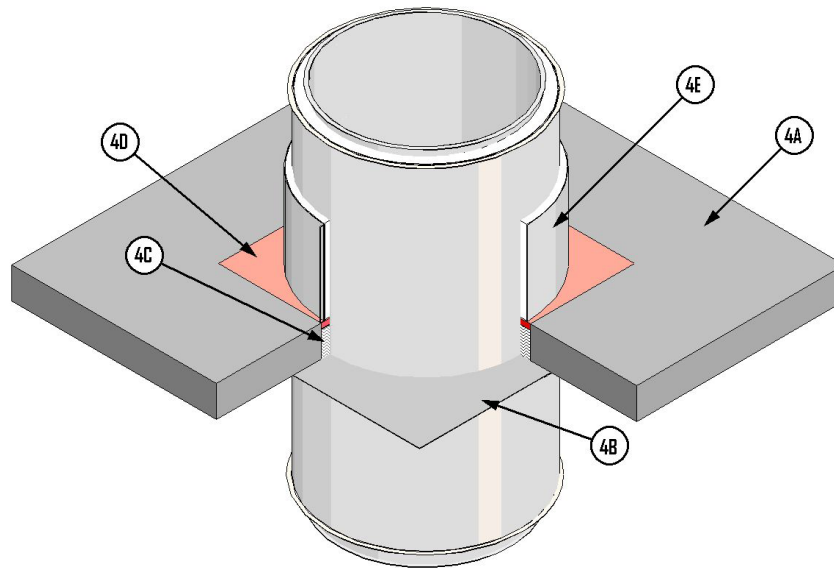
Figure 4. Floor/Ceiling Firestop
