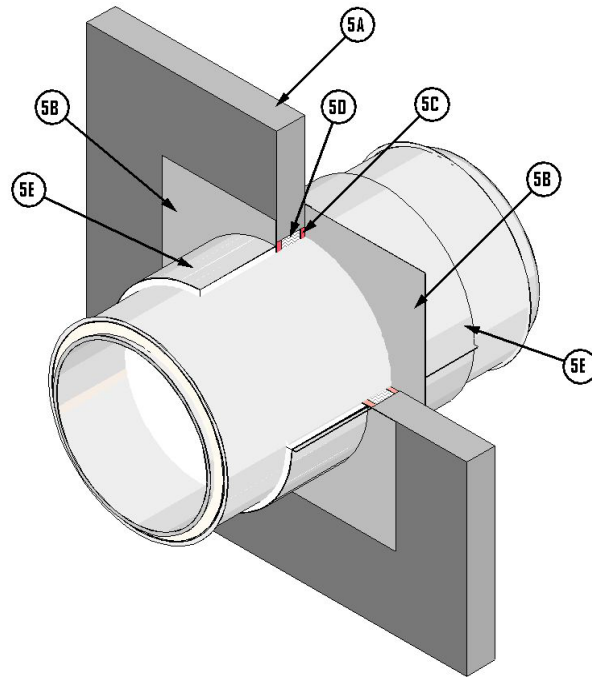
Figure 5. Wall Firestop
