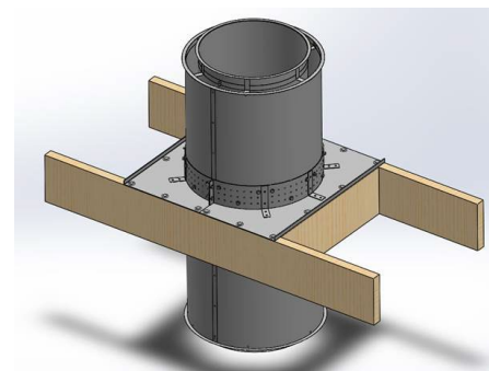
Floor Support Assembly
