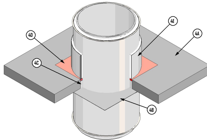
Figure 6: Floor/Ceiling Firestop
