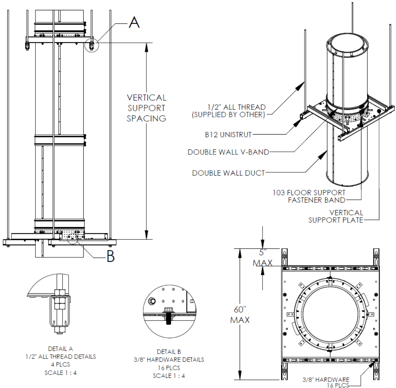
Figure 4. Floor/Ceiling Vertical Support Assembly – Suspended from Ceiling
