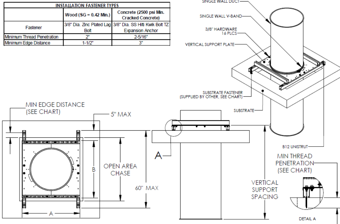
Figure 7. Floor Vertical Support Assembly
