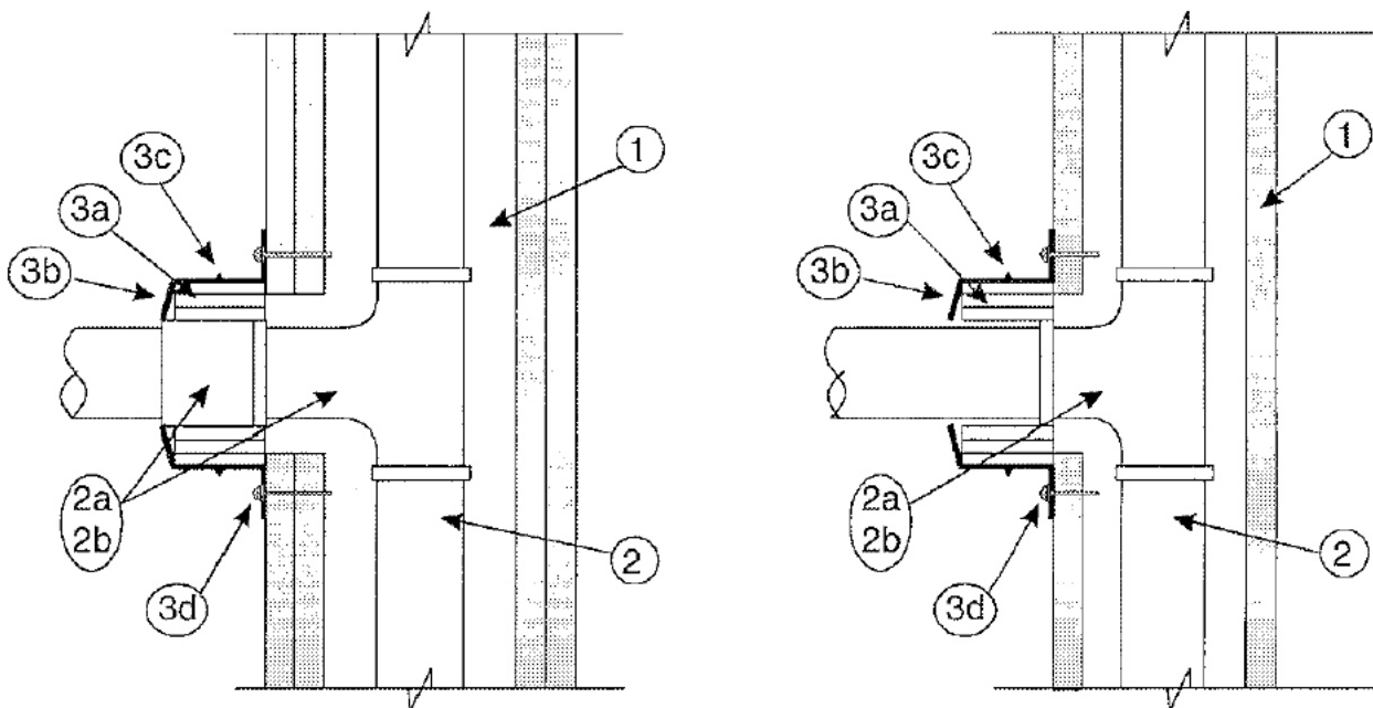
Figure 1. Penetration Detail
