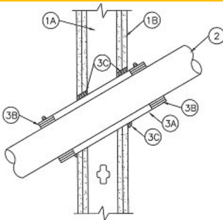
Figure 1. Penetration Detail
