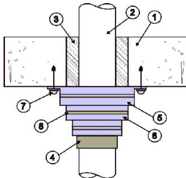
Figure 1. Penetration Detail
