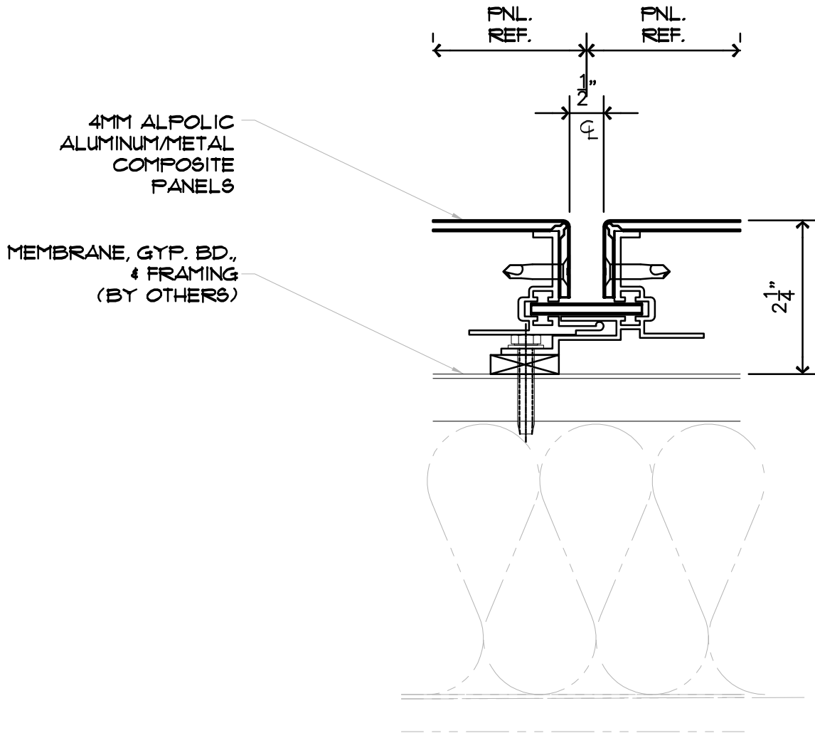
2 VERTICAL JOINT RS SCALE: 6" = 1'-0"
