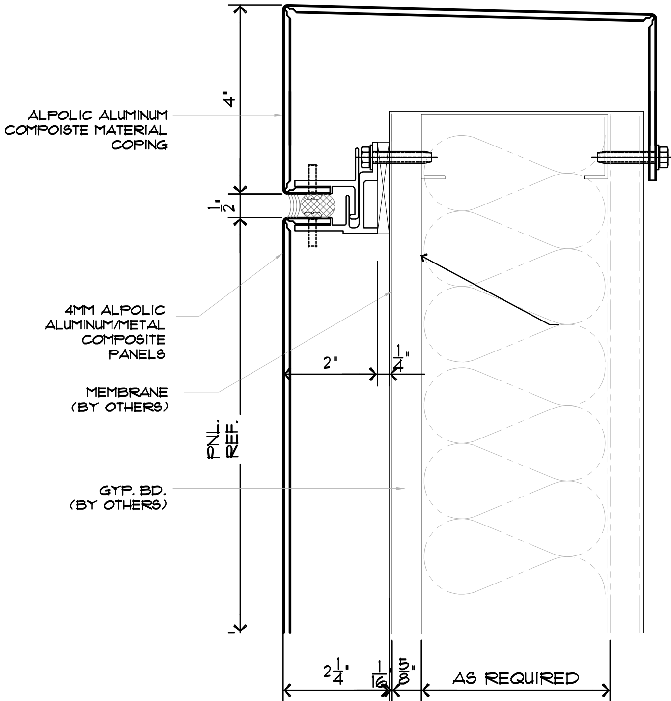
12 PARAPET DETAIL, OPTION 2 RS SCALE: 6" = 1'-0"
