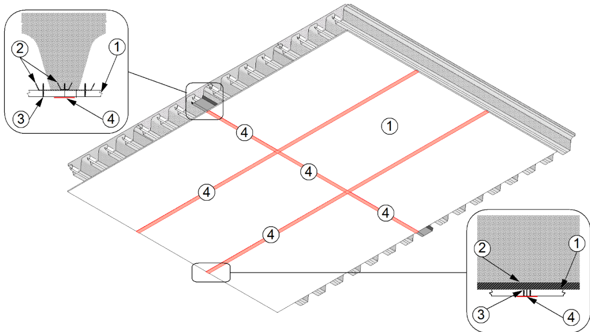
Figure 1 – Floor/Ceiling Assembly & Details
