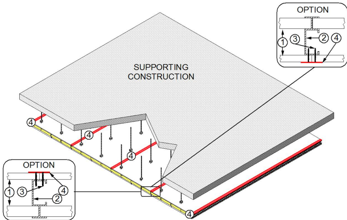
Figure 1 – Floor/Ceiling Assembly & Details
