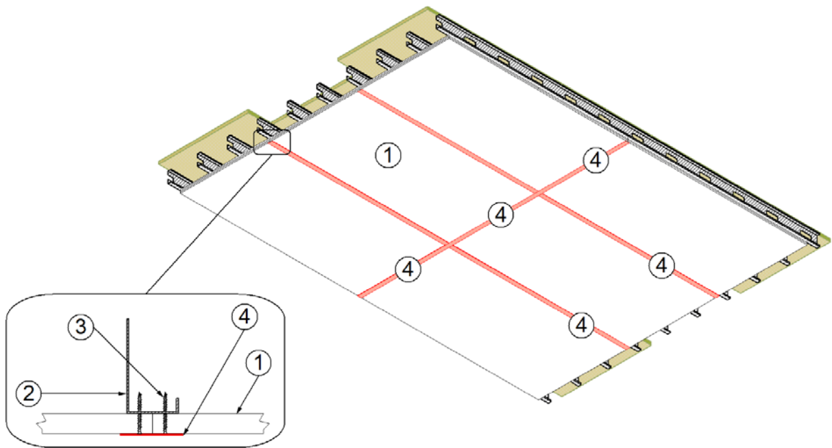
Figure 1 – Floor/Ceiling Assembly & Details
