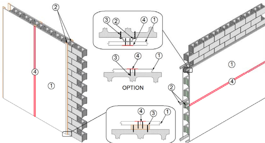
Figure 1 – Wall Assembly & Details
