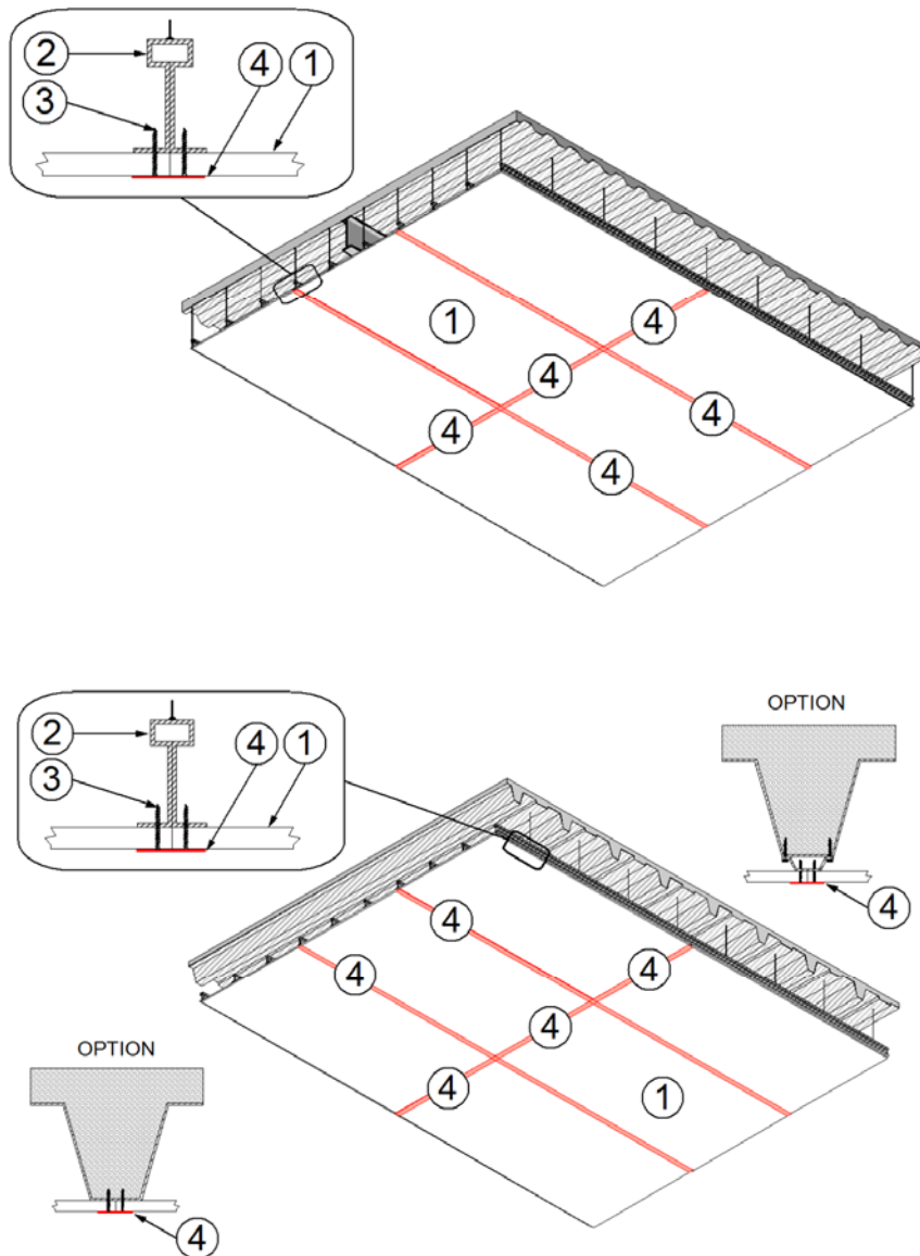
Figure 1 – Floor/Ceiling Assembly & Details
