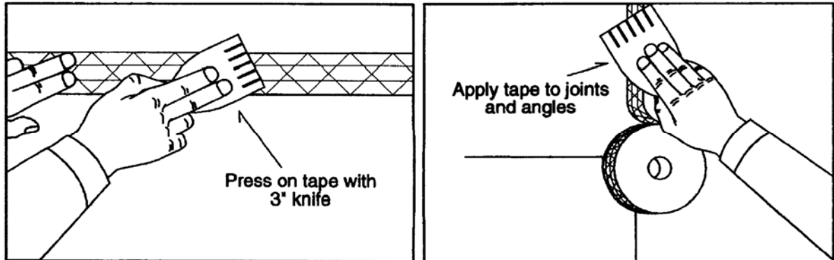
Figure 2 – Installation Methods
