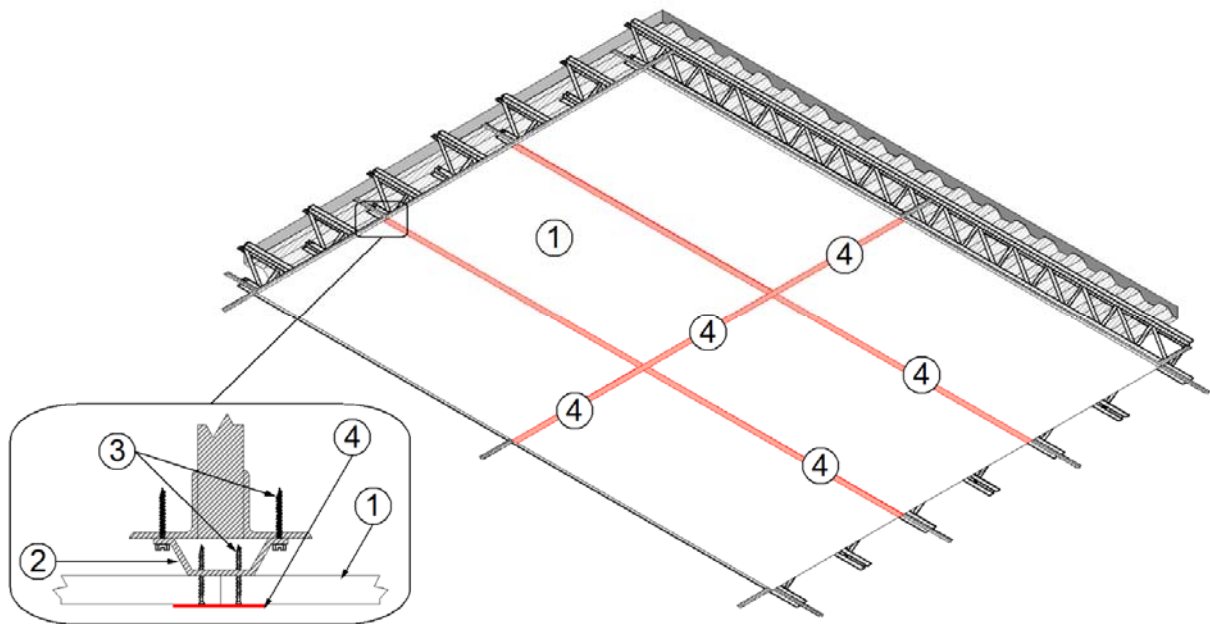
Figure 1 – Floor/Ceiling Assembly & Details
