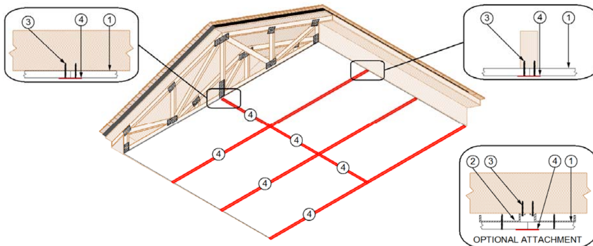
Figure 1 – Roof/Ceiling Assembly & Details
