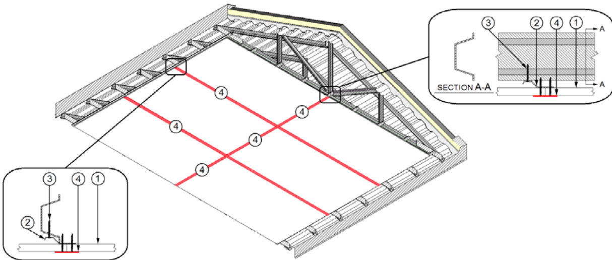
Figure 1 – Roof/Ceiling Assembly & Details
