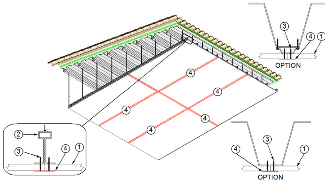
Figure 1 – Roof/Ceiling Assembly & Details
