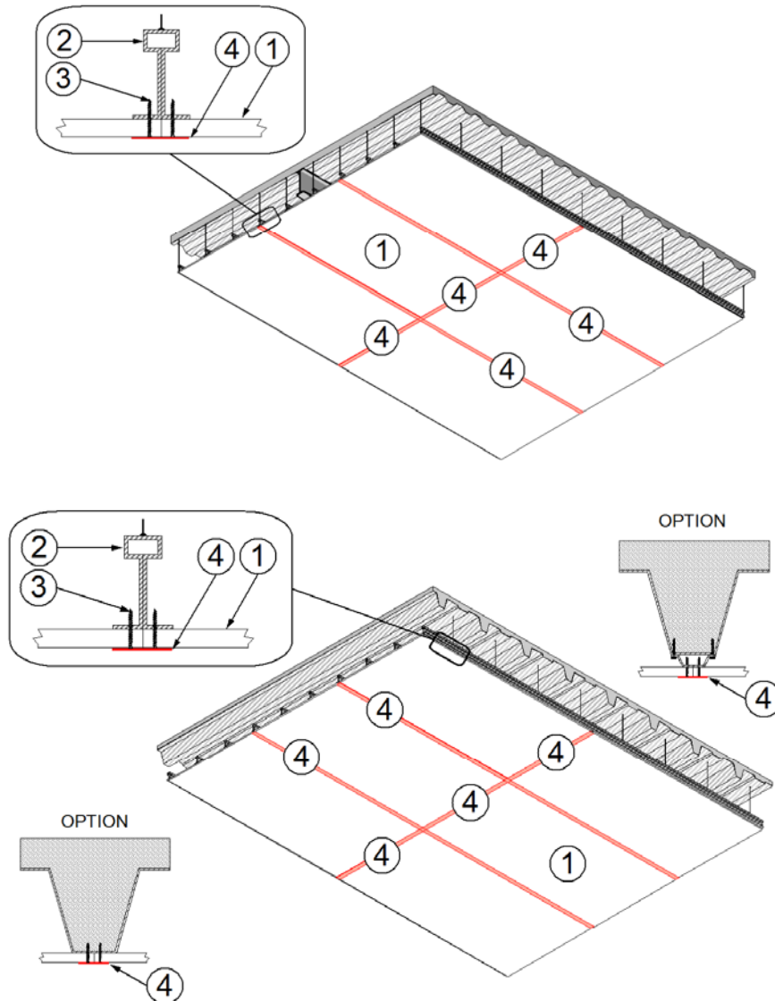
Figure 1 – Floor/Ceiling Assembly & Details
