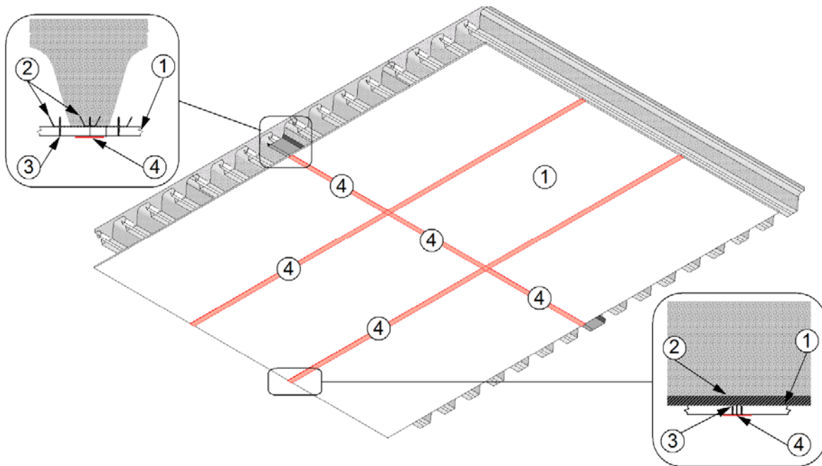
Figure 1 – Floor/Ceiling Assembly & Details
