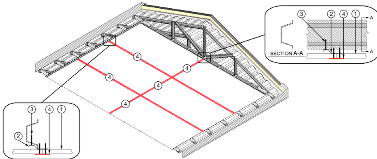
Figure 1 – Roof/Ceiling Assembly & Details
