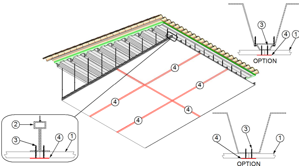
Figure 1 – Roof/Ceiling Assembly & Details
