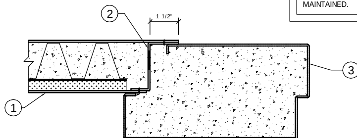
JAMB @ WIDE JAMB LOCK
