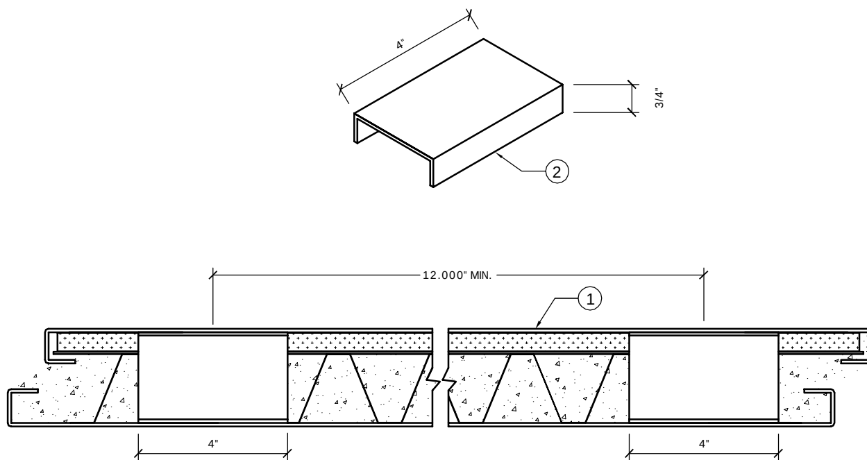
BOTTOM VIEW OF PANEL W/ CHANNELS INSTALLED
