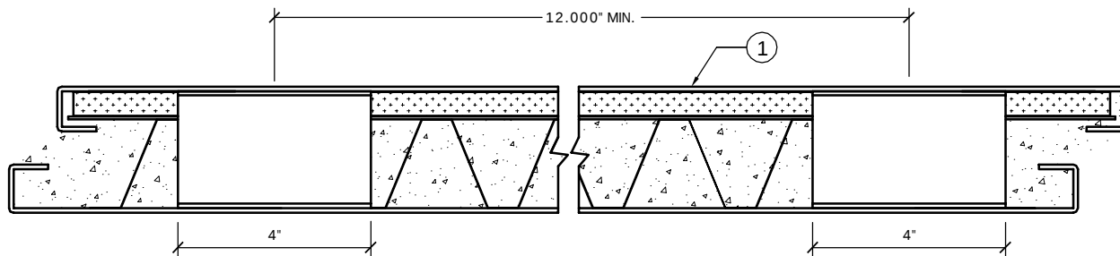
BOTTOM VIEW OF PANEL W/ CHANNELS INSTALLED
