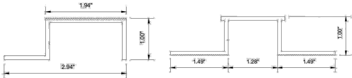
Figure 3 – J- and H-Section Studs
