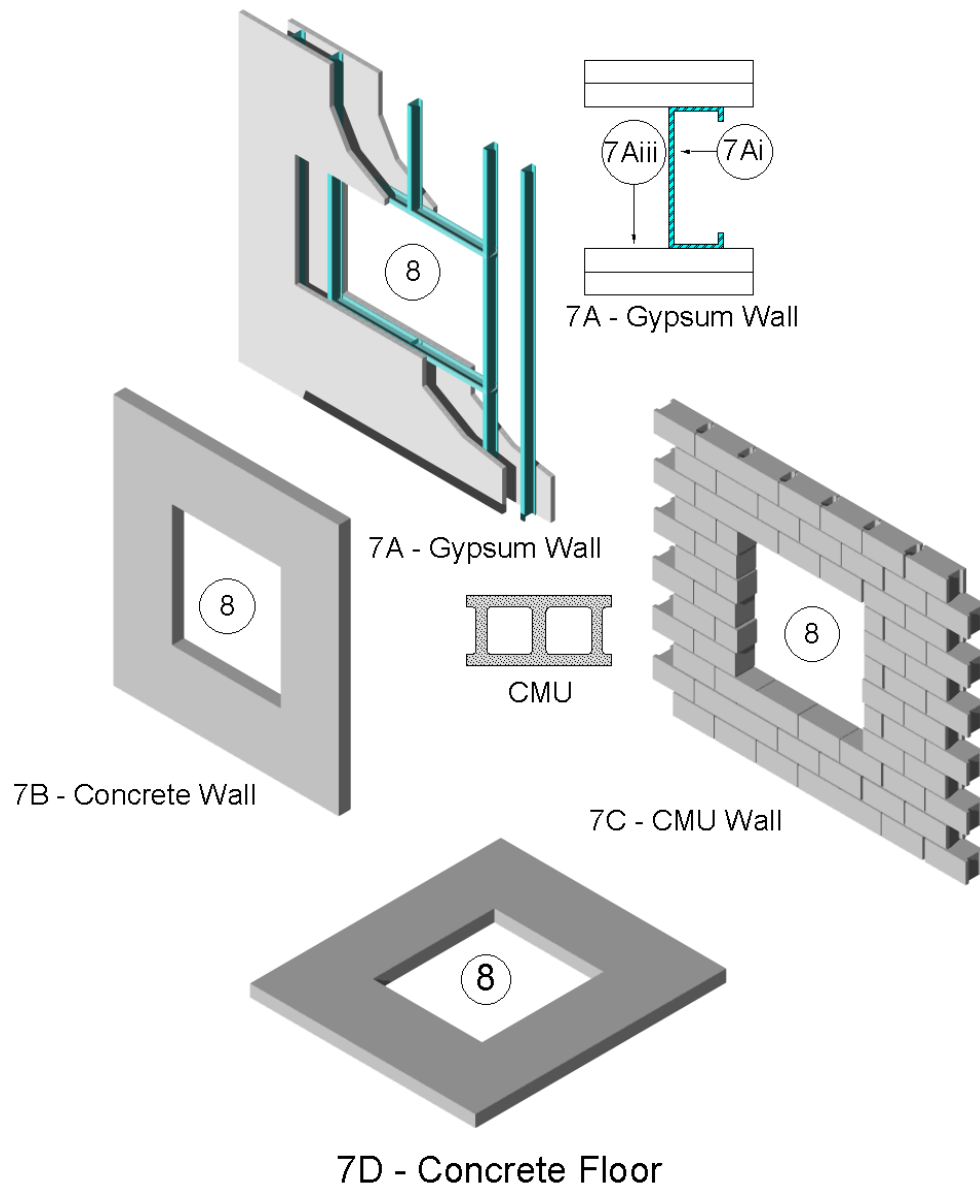
Figure 5 – Supporting Constructions
