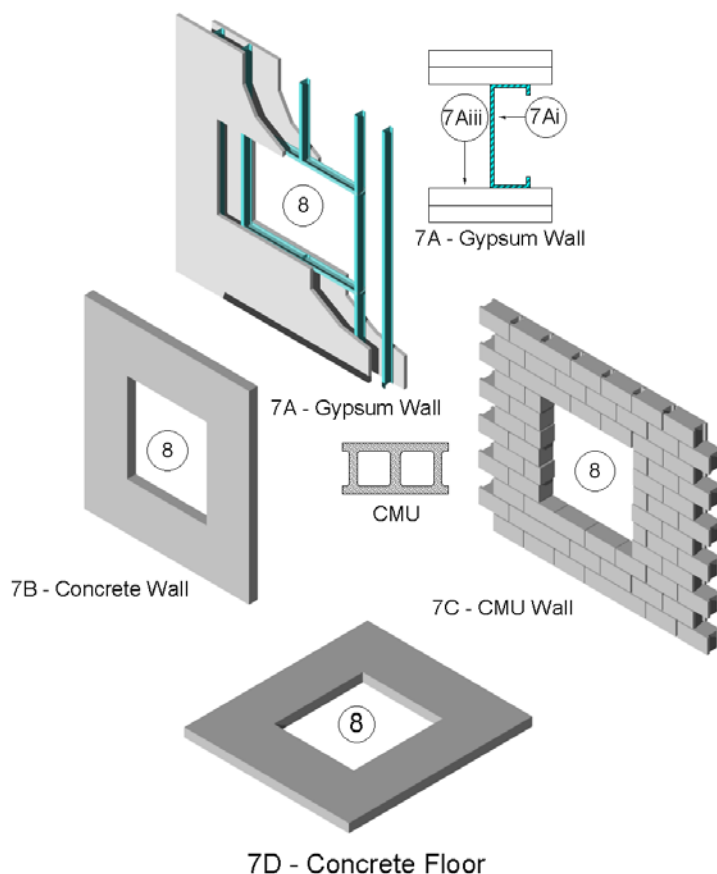
Figure 5 – Supporting Constructions
