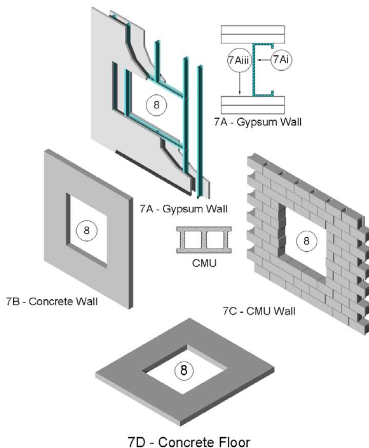
Figure 5 – Supporting Constructions
