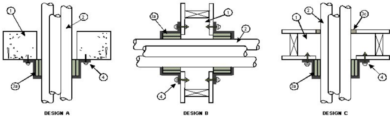
Figure 1. Penetration Detail
