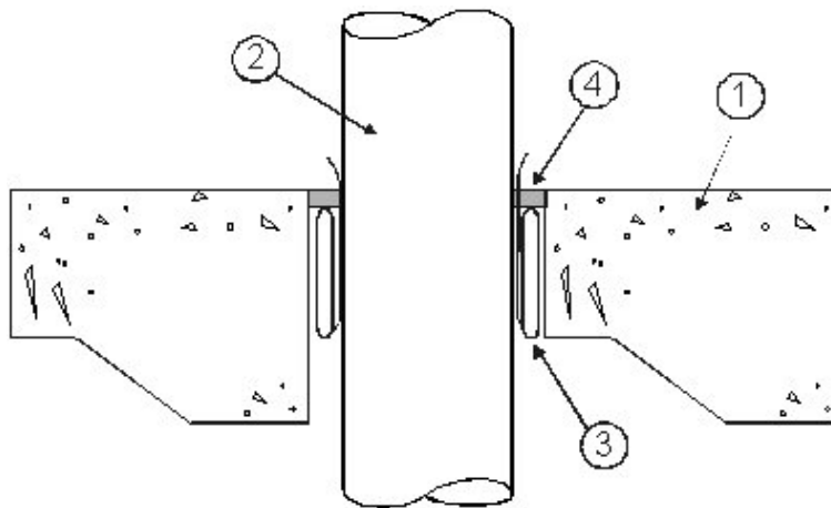
Figure 1. Penetration Detail
