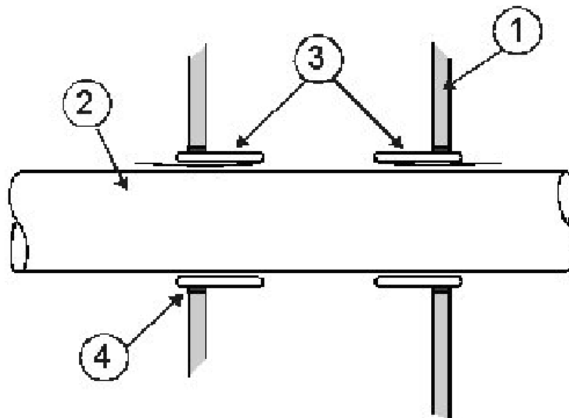
Figure 1. Penetration Detail
