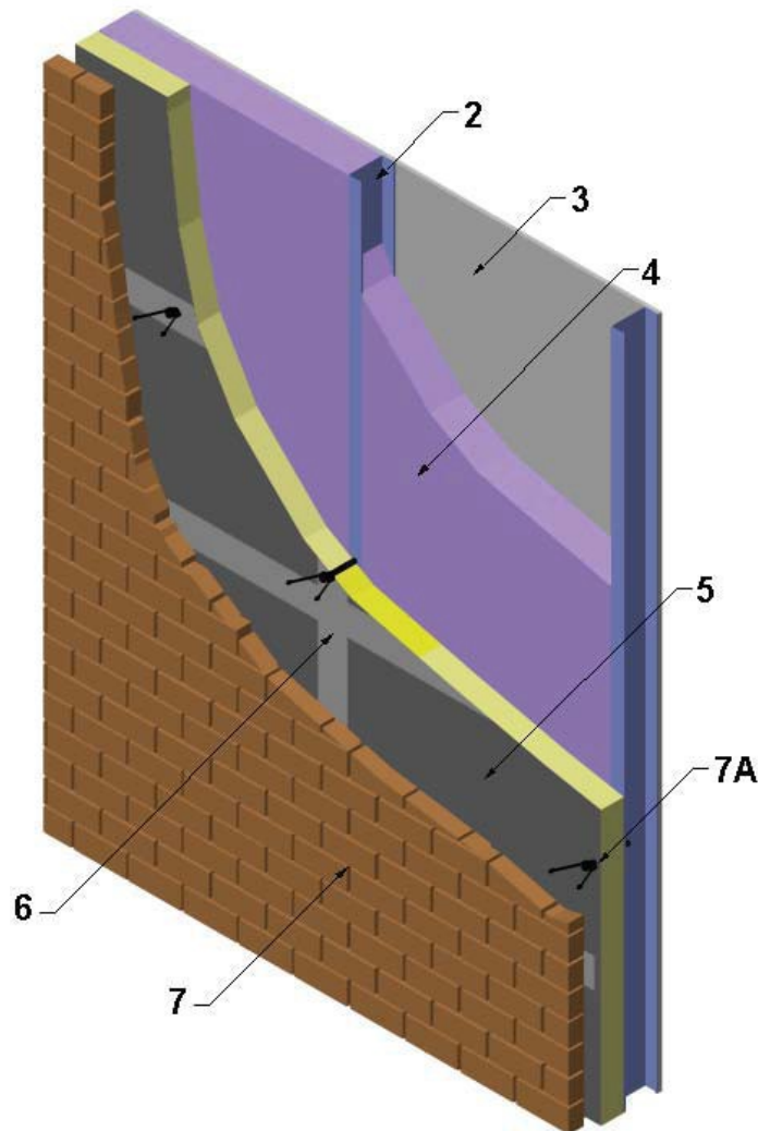
Item 1: Exterior Wall Assembly
