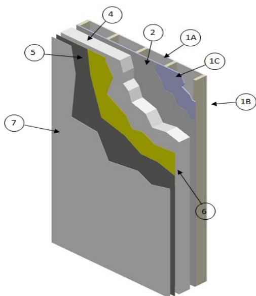
Figure 1: Construction with Wood Studs
