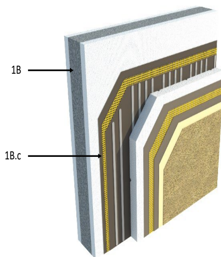
Figure 3: ICF Base Wall
