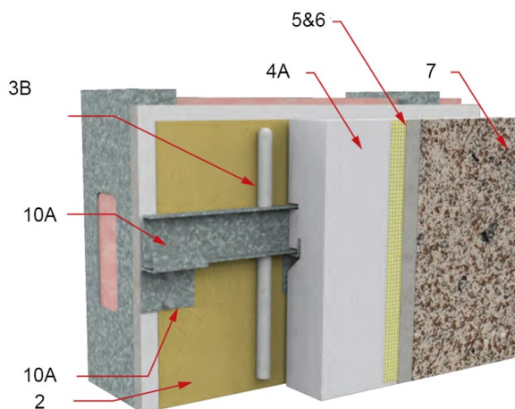
Figure 4: StoLite Panel and Mounting Method
