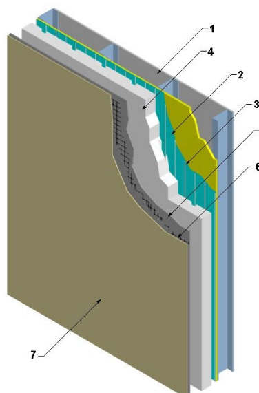
Figure 2: Construction with Steel Studs
