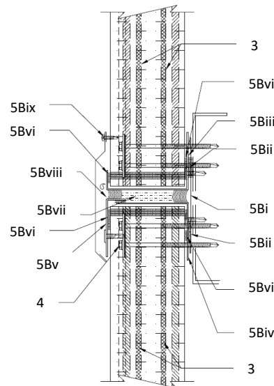
Stack Joint (Vertical)
