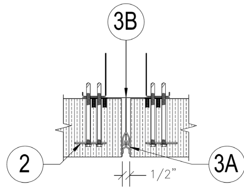
Butt Joint Detail
