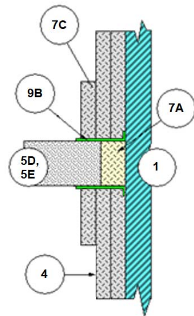
Floor Through Penetration Detail
