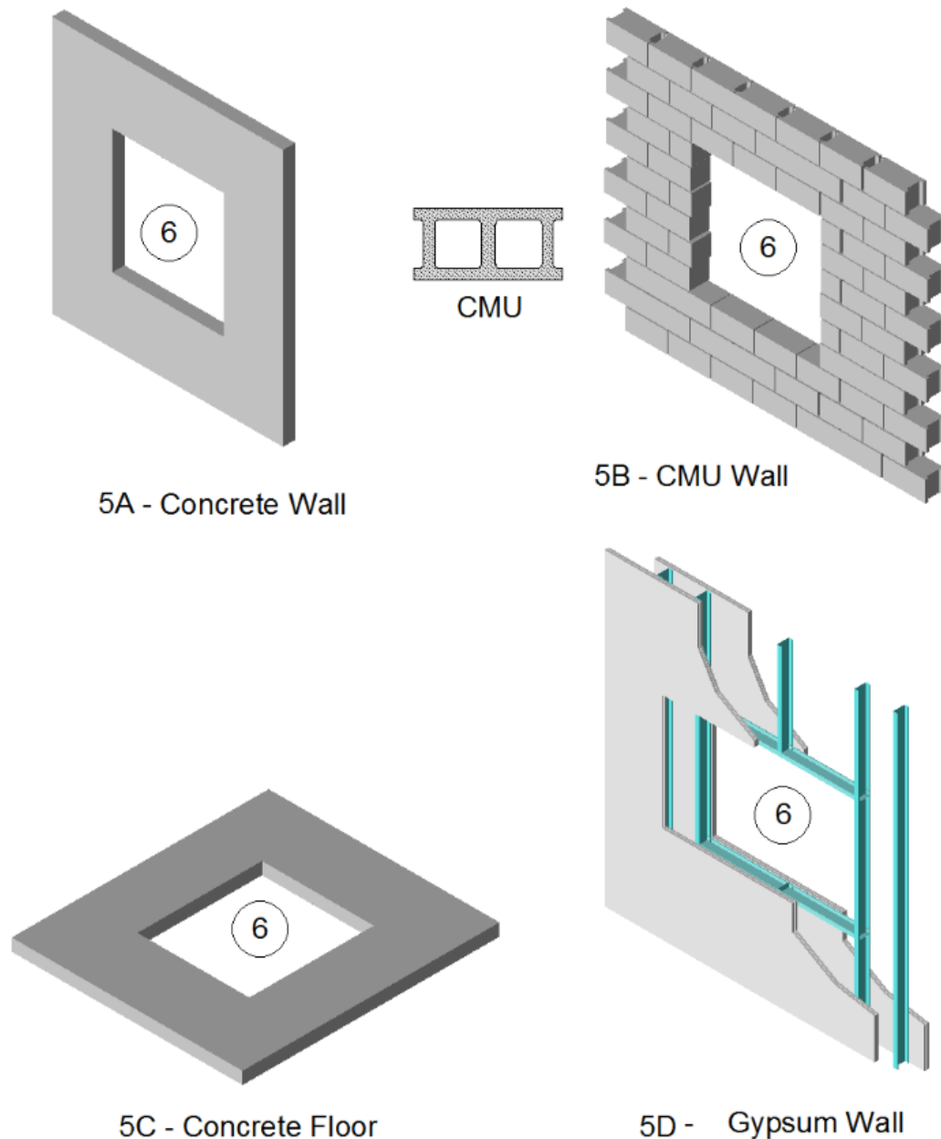
Figure 2. Supporting Construction.
